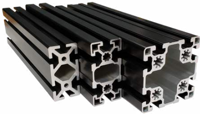
Extrusion (Fractional, Metric, B-Series)
